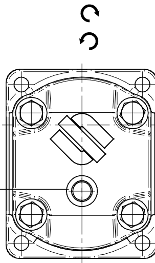
Standard rear cover for reversible pumps, with external drain C. For the dimension C please see the table here below
