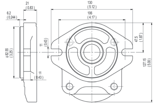
S2 SAE A 2 bolts
