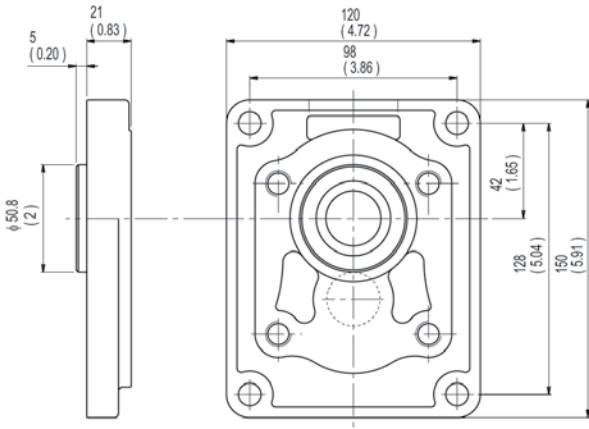
P2 European standard
