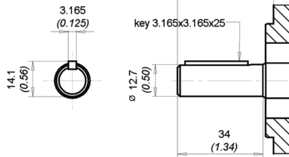
code 83 Max torque 40 Nm (354 lbf in) SAE Parallel
