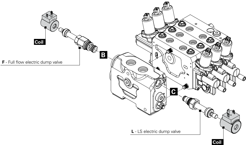
F - Full flow dump valve L - LS electric dump valve
