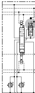
Electrohydraulic actuation
