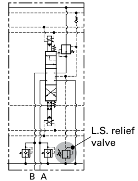
Electrohydraulic actuation
