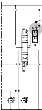
Mechanical lever actuation
